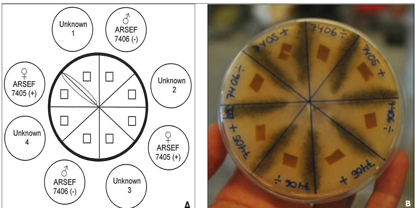
Fig. 5. Ascospheera apis mating test and production of inoculums. A. Mating test with four isolates of unknown mating types. Unknown 1 mates with ARSEF 7405 (+) and therefore harbours the opposite mating type (-). B. Production of inoculums between two isolates of opposite mating types. Fruiting bodies with spores inside are formed where the hyphae meet (black zone). Photo: A B Jensen
