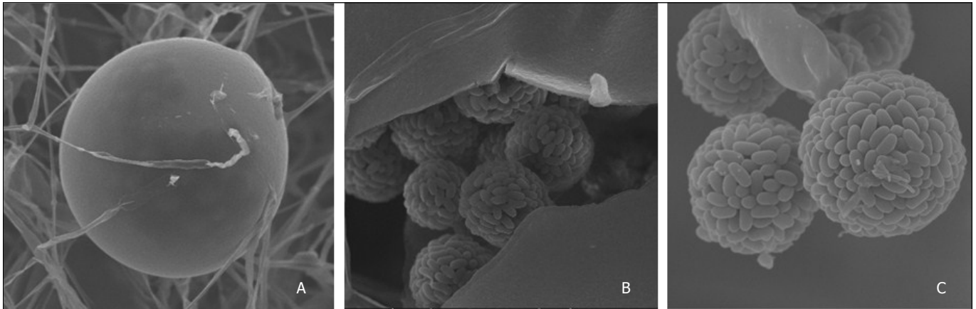
Fig. 3. Scanning electron microscope pictures of Ascospheara apis fruiting body. A. Spherical fruiting body; B. Cracked fruiting body with sporeballs; C. Sporeballs with multiple ascospores. Photos: J Bresciani and A B Jensen
